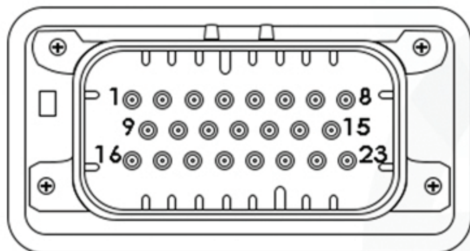
23-PIN AMPSEAL CONNECTOR PIN-OUT DIAGRAM
